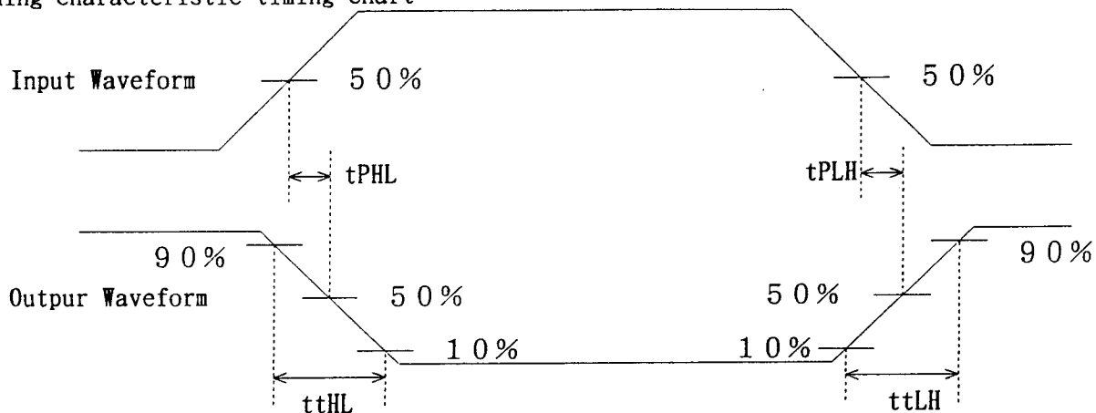
Switching characteristic timing chart
